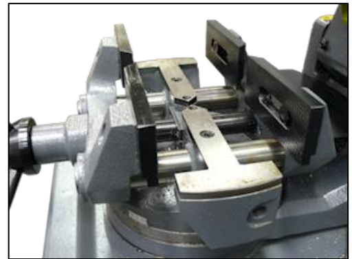
Self-centring Vice
