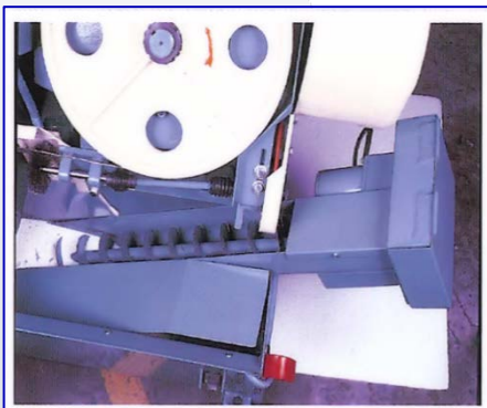
Swarf conveyor
