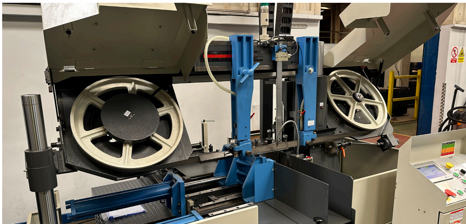
Hydraulic Top Clamps
