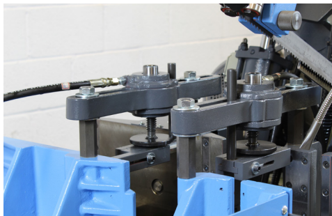
Hydraulic Top Clamps
